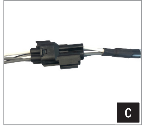
C. Connect the front (white/gray) output from the MR1 power harness to the B-H1909 front speaker harness.
