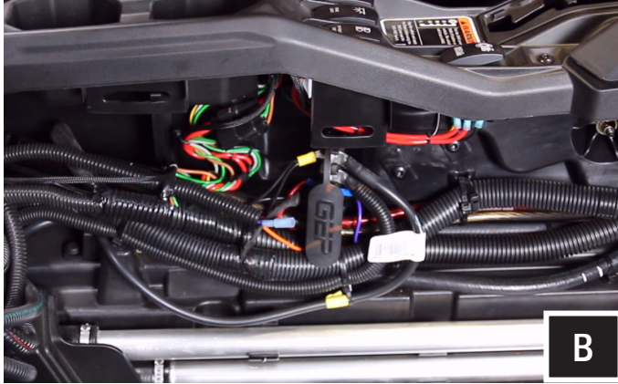
B. Zip tie all wiring to the factory cables away from any moving parts.
