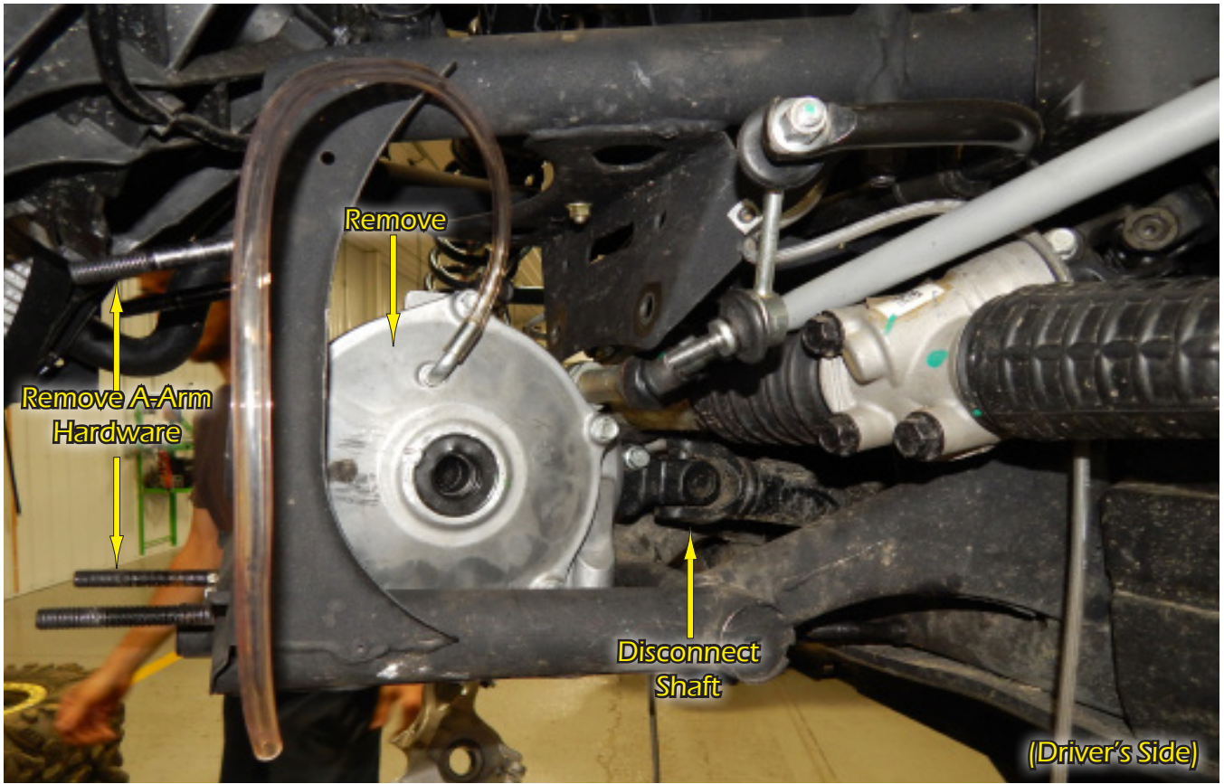
7. Remove Axles, Front Differential, and Hardware as shown in Fig.7.
