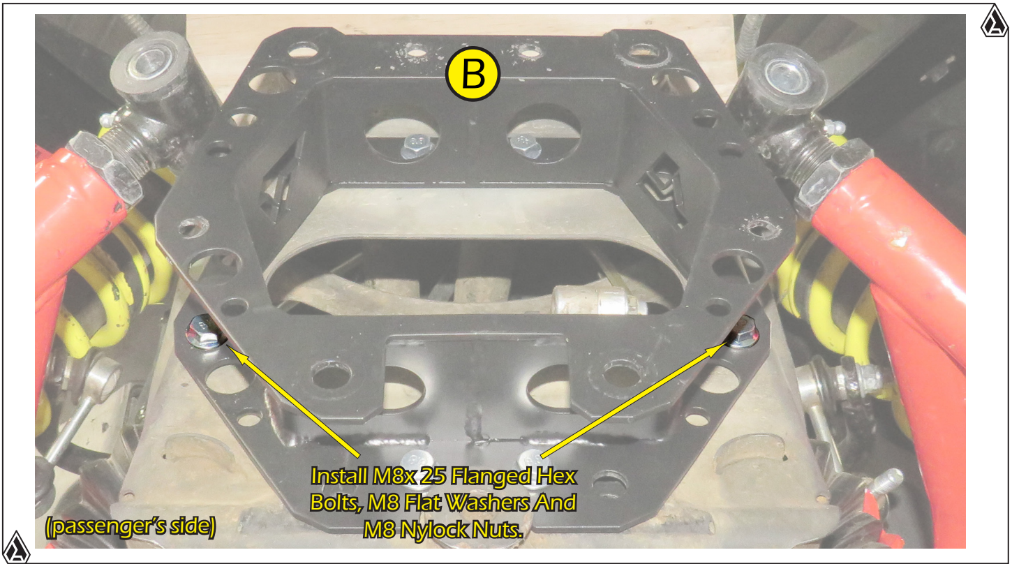
16. Secure Mount (B) with hardware shown. Hardware should be snug but not tight. See Fig. 16 . FIG. 16
