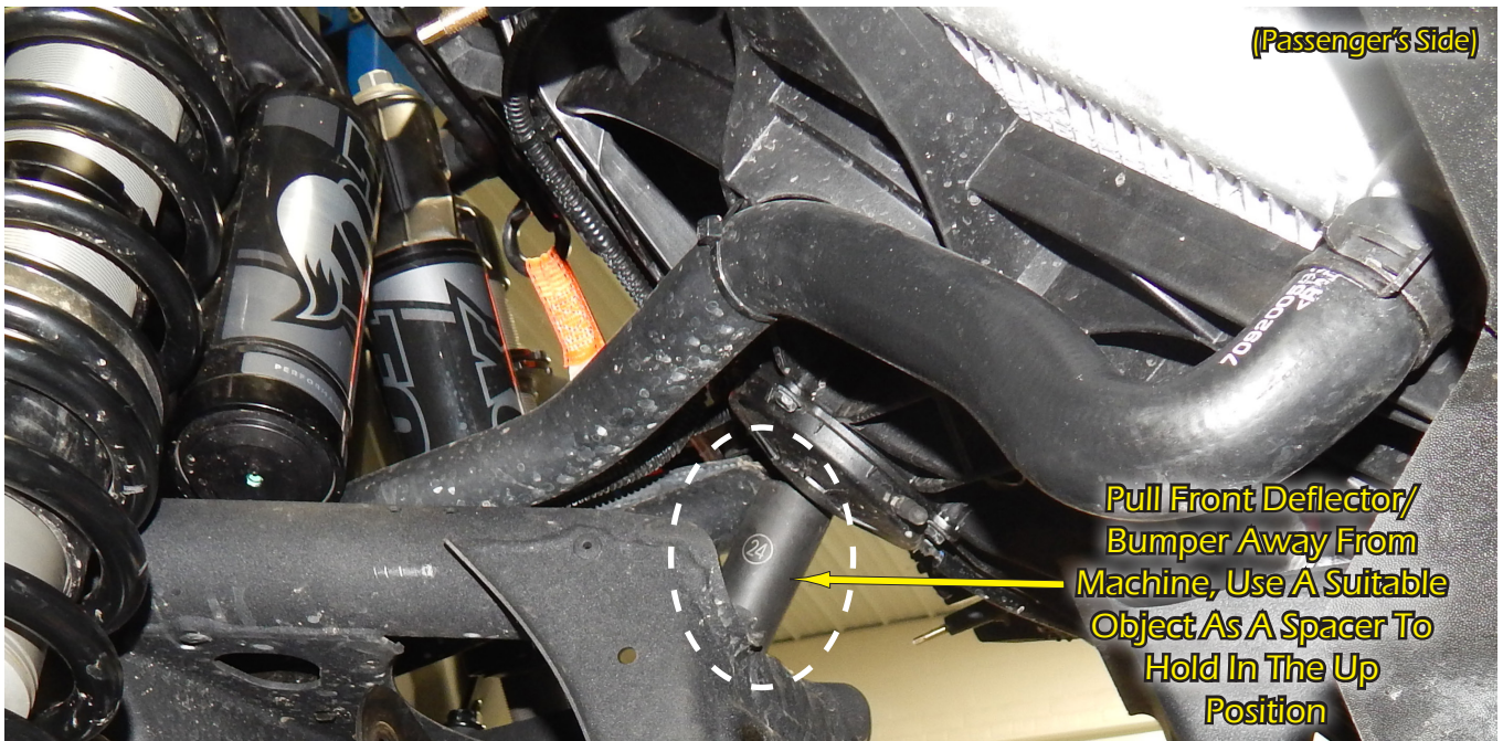
6. Remove A-Arms from machine. See Fig.6.
