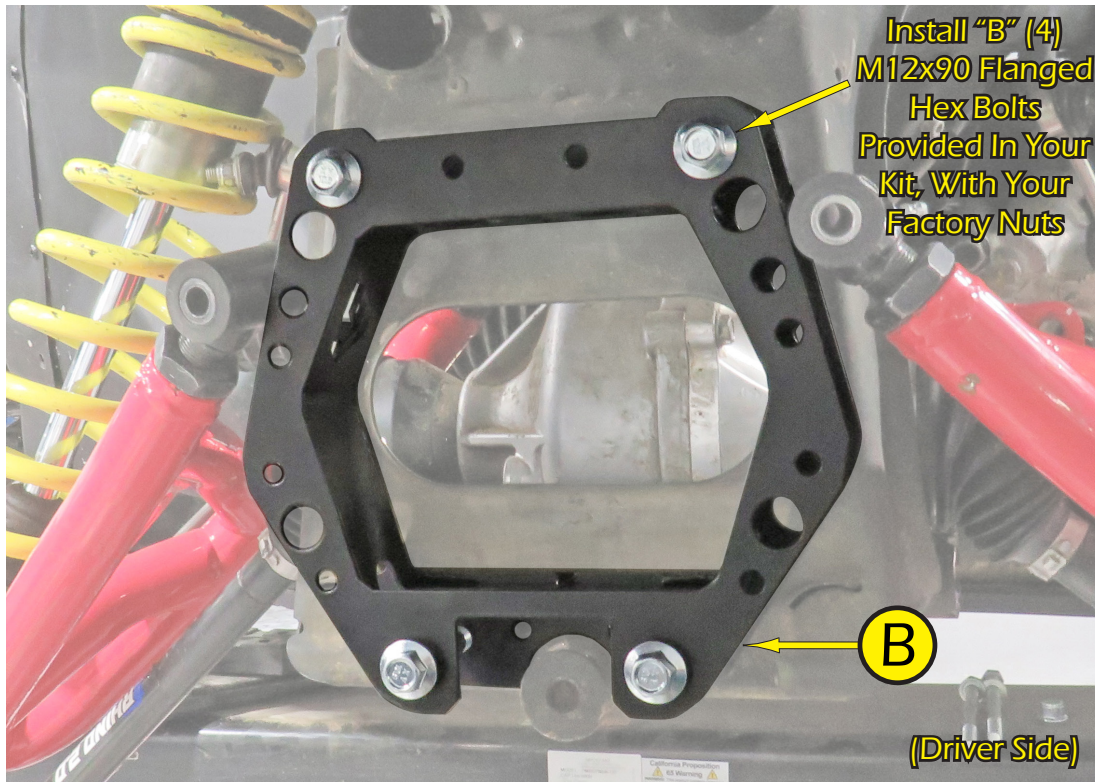
10. Install Mount (B) with hardware shown. Hardware should be snug but not tight. See Fig.10.
