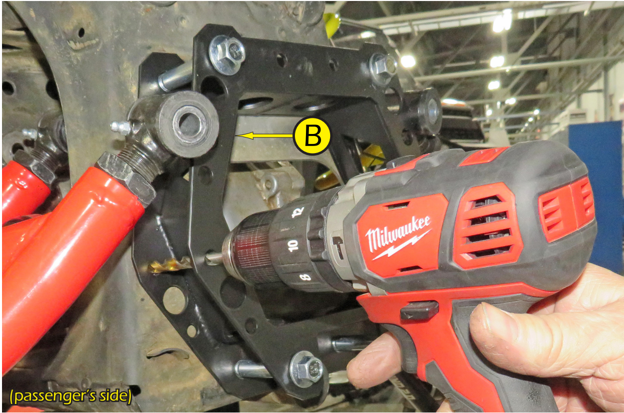
11. Drill (4) holes through Frame. Holes must be large enough for Ø8mm bolts. See Fig.11.
