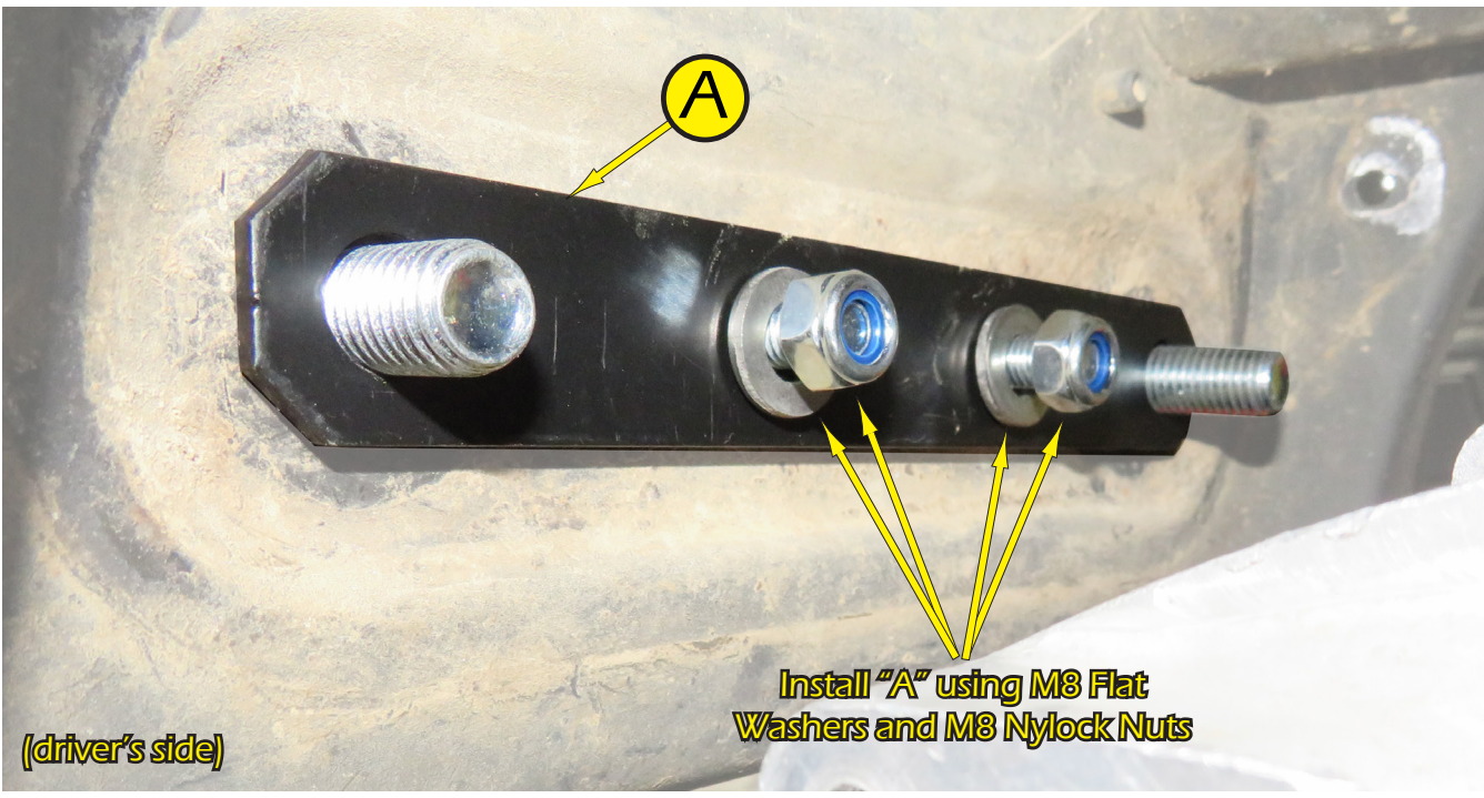
13. Then install Upper Plate to those bolts using M8 Flat Washers and M8 Nylock Nuts. Hardware should be snug but not tight. See Fig.13.
