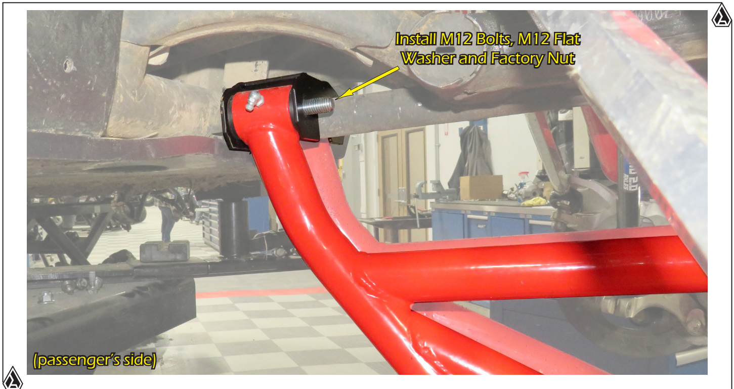
21. Secure Lower A-Arms to Shear Plate (F), Frame, and Lower Brace (D) with hardware shown. See Fig.21.
