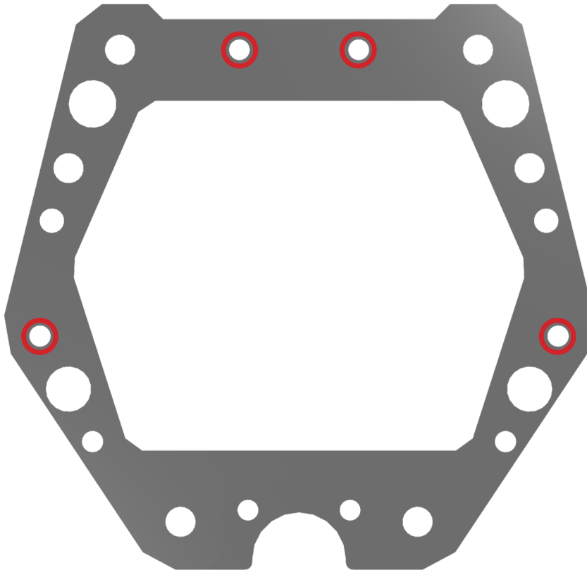
11. Drill (4) holes through Frame. Holes must be large enough for Ø8mm bolts. See Fig.11.
