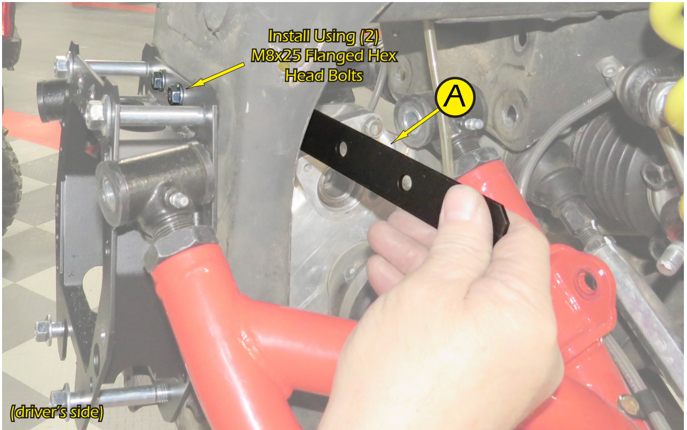
12. Install Mount Using (2) M8x25 Flanged Hex Head Bolts. See Fig.12.
