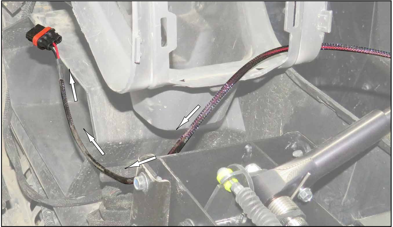
route Harness to Center Storage area (see pages 9 and 12)
