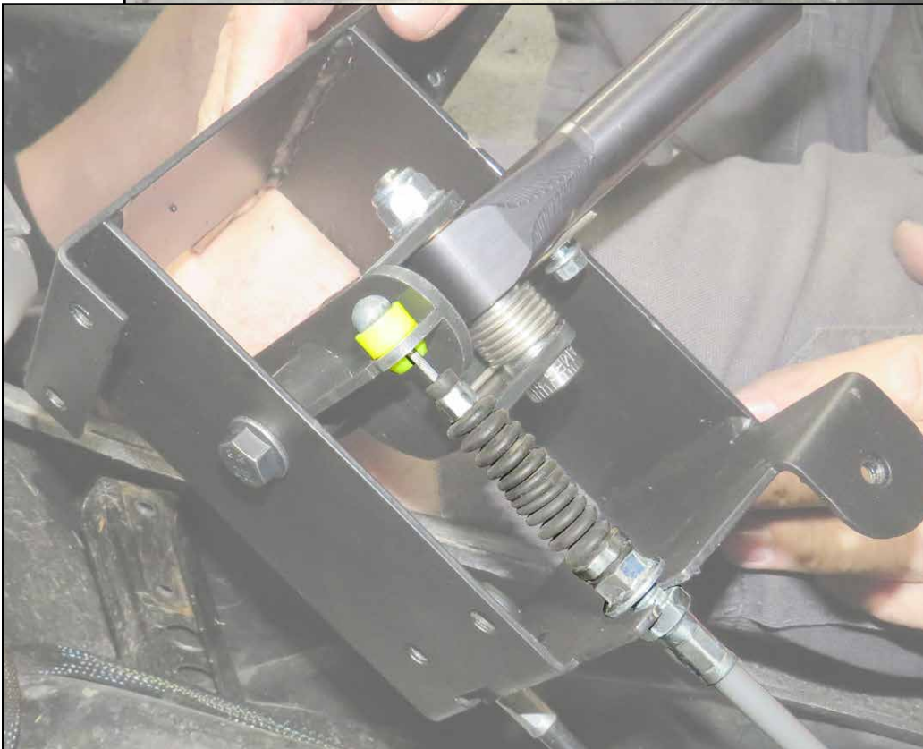
Tighten Shifter Cable Nuts
