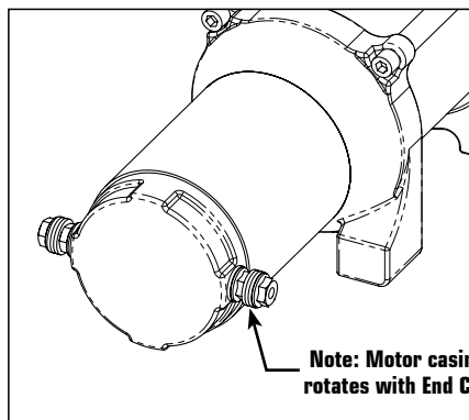
LEADS ROTATED 90°
