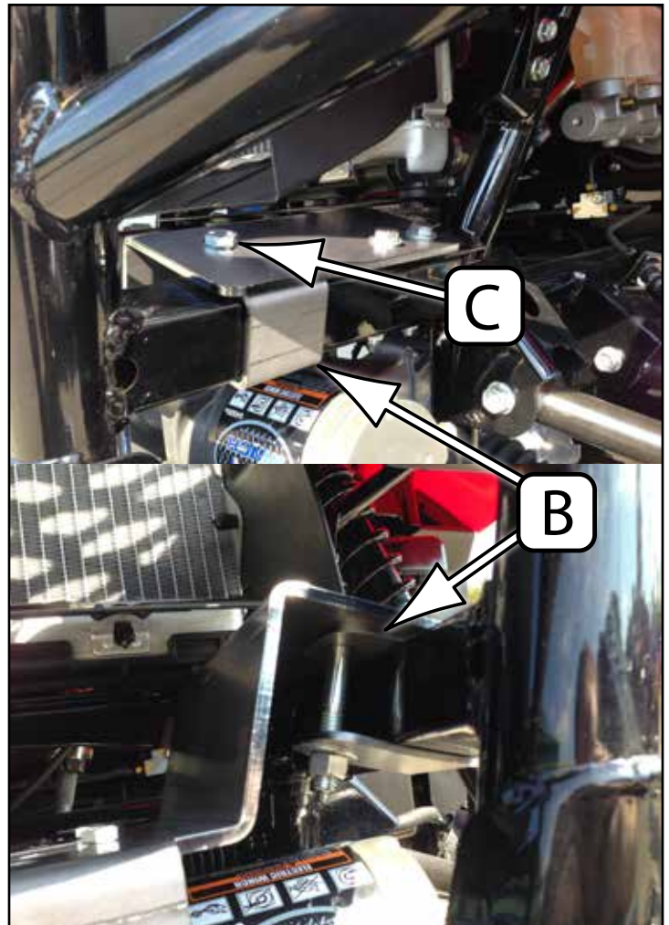
“Figure 5 Mount and Bracket Install to Bumper” (Bumper shown attached to frame, the bumper should not be attached at this time.)
