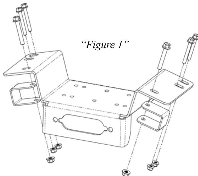
Standard 4 Hole Winch Pattern (4.875" x 3")
