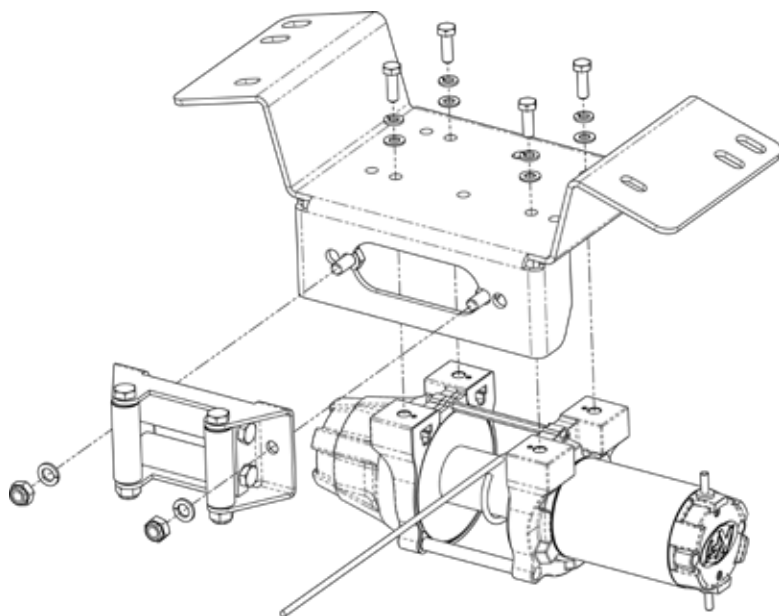
"Figure 3 Winch Install"
