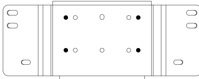
Wide 4 Hole Winch Pattern (6.6" x 3")
