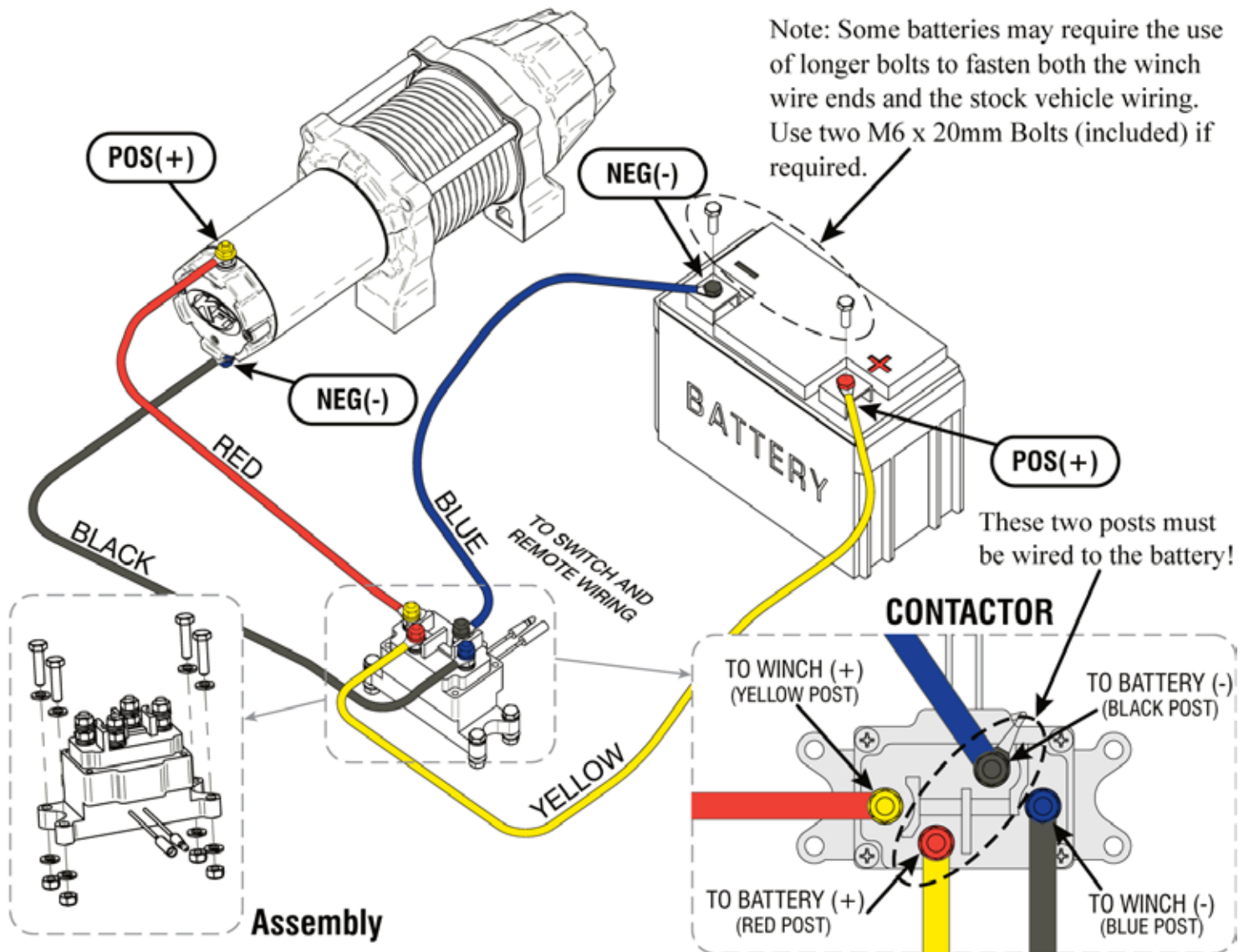
"Figure 10" Alternate Wiring Diagram
