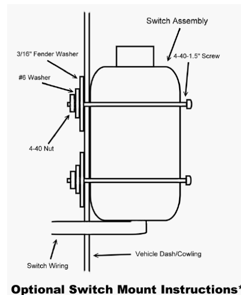
"Figure 8" Mini-Rocker Mounting
