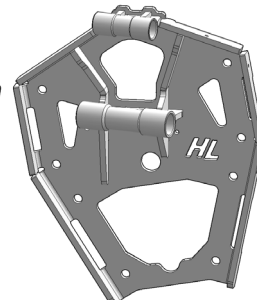
73-16004-R Right Rear Portal Backing Plate (1ea)
