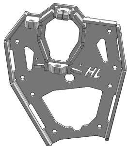
73-16008-L Left Front Portal Backing Plate (1ea)
