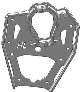
73-16008-R Right Front Portal Backing Plate (1ea)
