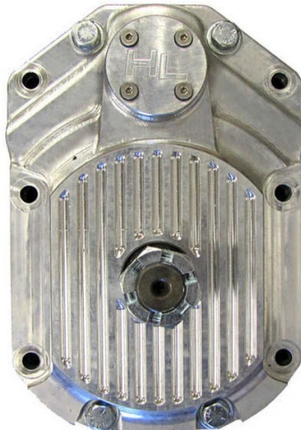
Assembled Portal Box (4ea) PGLAB-645-P603
